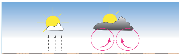
Convection
